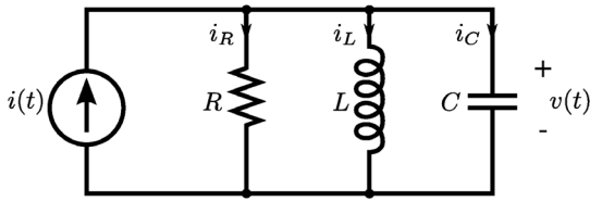
Figure 5. A parallel RLC circuit, with source. We can use the established rules to write the Lagrangian function for the circuit as: \mathcal{L} = +(jR/2)(i_R^{(-1/2)})^2 + (L/2)(i_L^{(0)})^2 - (1/(2C))(i_C^{(-1)})^2 . We also use Kirchhoff's current law to impose a constraint function of \Psi = i_R + i_L + i_C - i_S = 0 , and we use the principle of the Lagrange multiplier to obtain an ordinary differential equation to describe the dynamical behaviour of v(t) . doi:10.1371/journal.pone.0077190.g005
