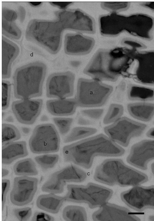
Fig. 1. SEM backscattered electron (BSE) image of coralline algae (sample 302) showing detail of magnesite cell infill ( a, b ) and protodolomite rims ( e ) within Mg-calcite cell wall structure ( d ). Black lines and textures within the cells are most likely voids or remnant organic structures. Above “d” micron scale bands of slightly darker grey within the cell walls indicate varying magnesium within the cell wall. Concentric zonation is seen around cells (top left). SEM-EDS spot analyses of labeled sites a = 99.22, b = 99.19, c = 23.9, d = 15.17, e = 45.75 mol % \text{MgCO}_3 . Scale bar = 5 \mu\text{m} . ■ Cell wall structure (Mg-calcite 8–25 mol % \text{MgCO}_3 ) ■ protodolomite (38–62 mol % \text{MgCO}_3 ), ■ magnesite (95–99.55 mol % \text{MgCO}_3 ), ■ void.
