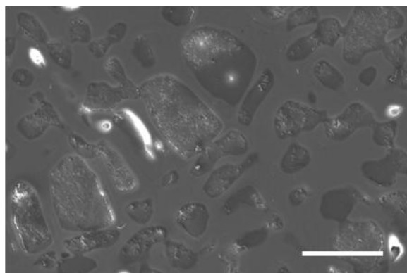
Fig. 6. SEM (SE) images showing the difference in cell in-fill between the top layers and the lower layers of coralline algae (sample 47). White indicates void (caused by charge build-up in sample) and shades of dark grey are in-fill. Top image taken at base of photosynthetically active layer, 0.5 mm from top of sample, showing that most cells are empty. Scale bar = 25 \mu m. Bottom image taken at 4 mm depth, showing abundant cell in-fill. There was a general, although patchy trend for increasing cell in-fill towards the base.
