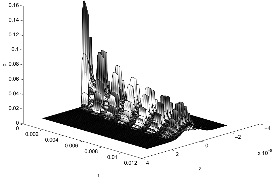
FIGURE 3. A finite-difference simulation of a Brownian ratchet, based on Parrondo's games. z is space, t is time and p is probability density. The spatial period of this ratchet is L_z = 2 \mu\text{m} . The temporal period of this ratchet is T_0 = 1.5 \text{ ms} . The physical constants are scaled for the diffusion of hydrated sodium ions in water.
