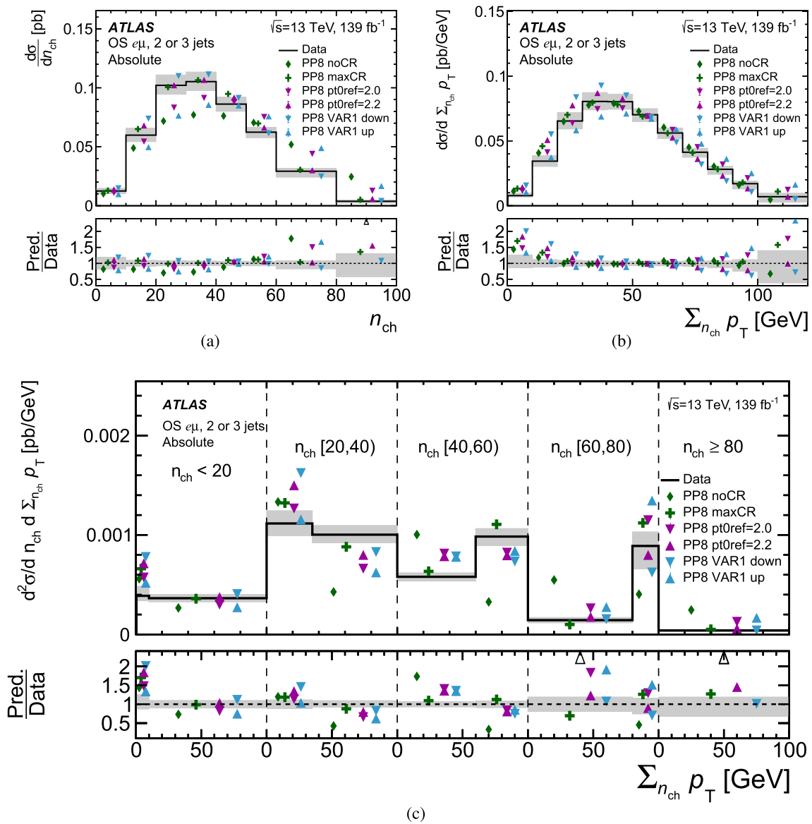
Fig. 18 Absolute differential cross-section as a function of a n_{ch} , b \sum_{n_{ch}} p_T , and c \sum_{n_{ch}} p_T in bins of n_{ch} . Unfolded data are shown as the black line with the grey band corresponding to the total uncertainty in each bin. The results are compared with the predictions of different CR and UE parameter variations in PYTHIA8. Events beyond the x -axis
