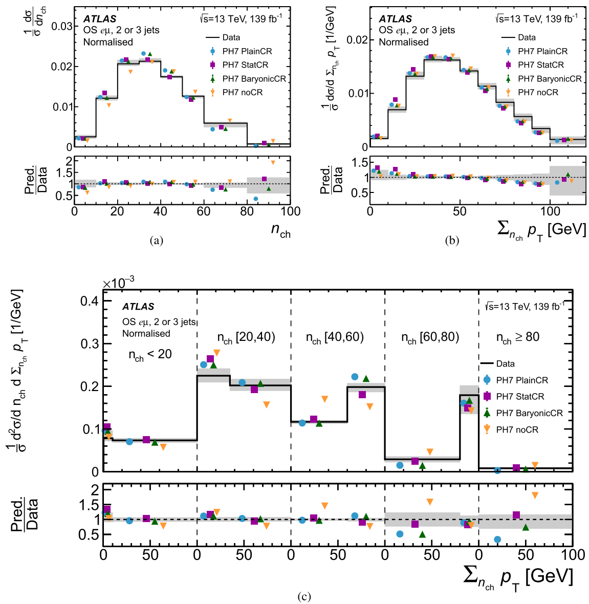
Fig. 13 Normalised differential cross-section as a function of a n_{ch} , b \sum_{n_{ch}} p_T , and c \sum_{n_{ch}} p_T in bins of n_{ch} . The x -axis in c is split into five bins of n_{ch} by the dashed vertical lines and \sum_{n_{ch}} p_T is presented in each bin. Unfolded data are shown as the black line with the grey
