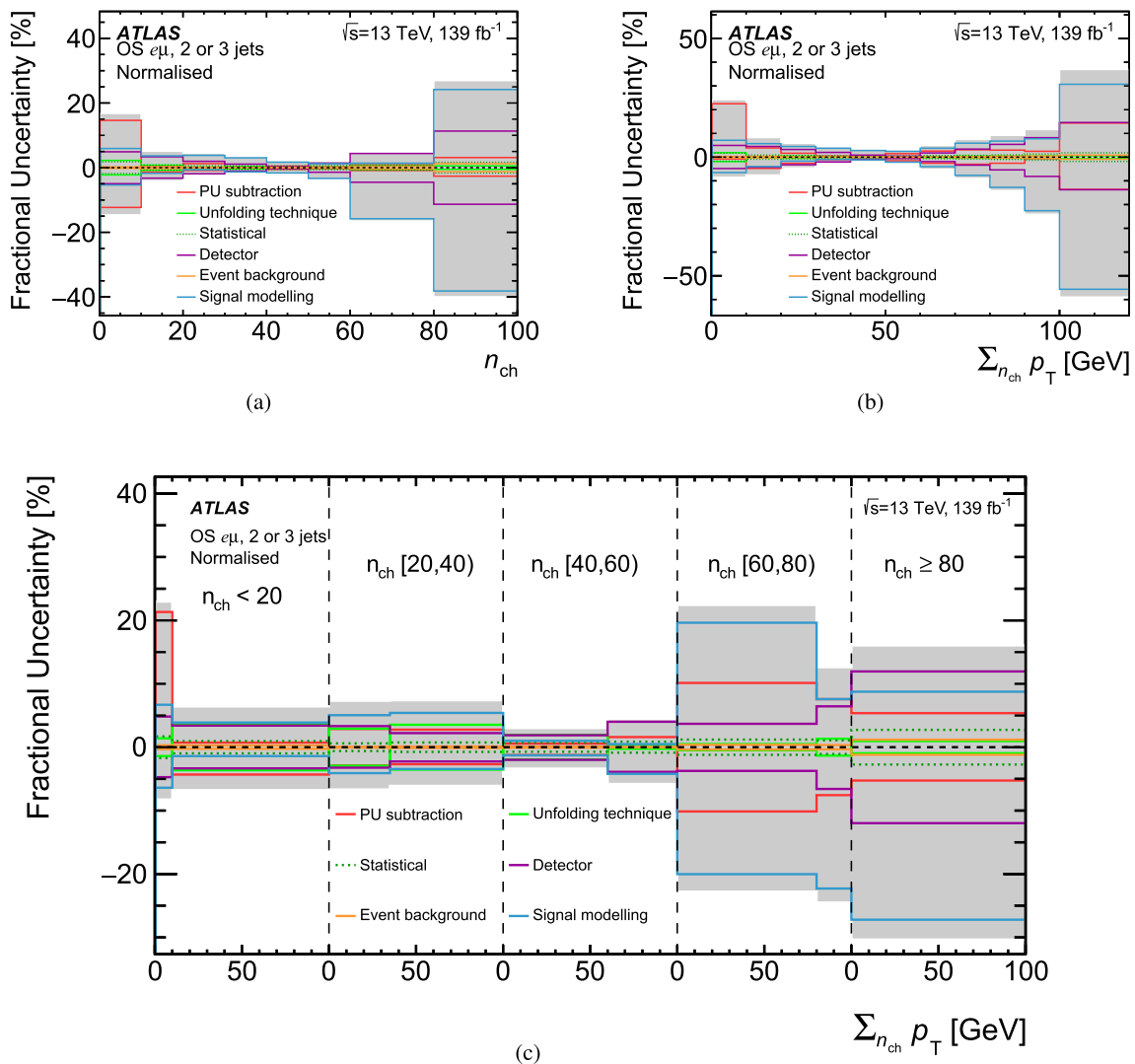
Fig. 8 Fractional uncertainties in the measured normalised differential cross-section as a function of a n_{\text{ch}} , b \sum n_{\text{ch}} p_T , c \sum n_{\text{ch}} p_T in bins of n_{\text{ch}} for all systematic and statistical uncertainties. The x -axis in c is split into five bins of n_{\text{ch}} by the dashed vertical lines and \sum n_{\text{ch}} p_T is
