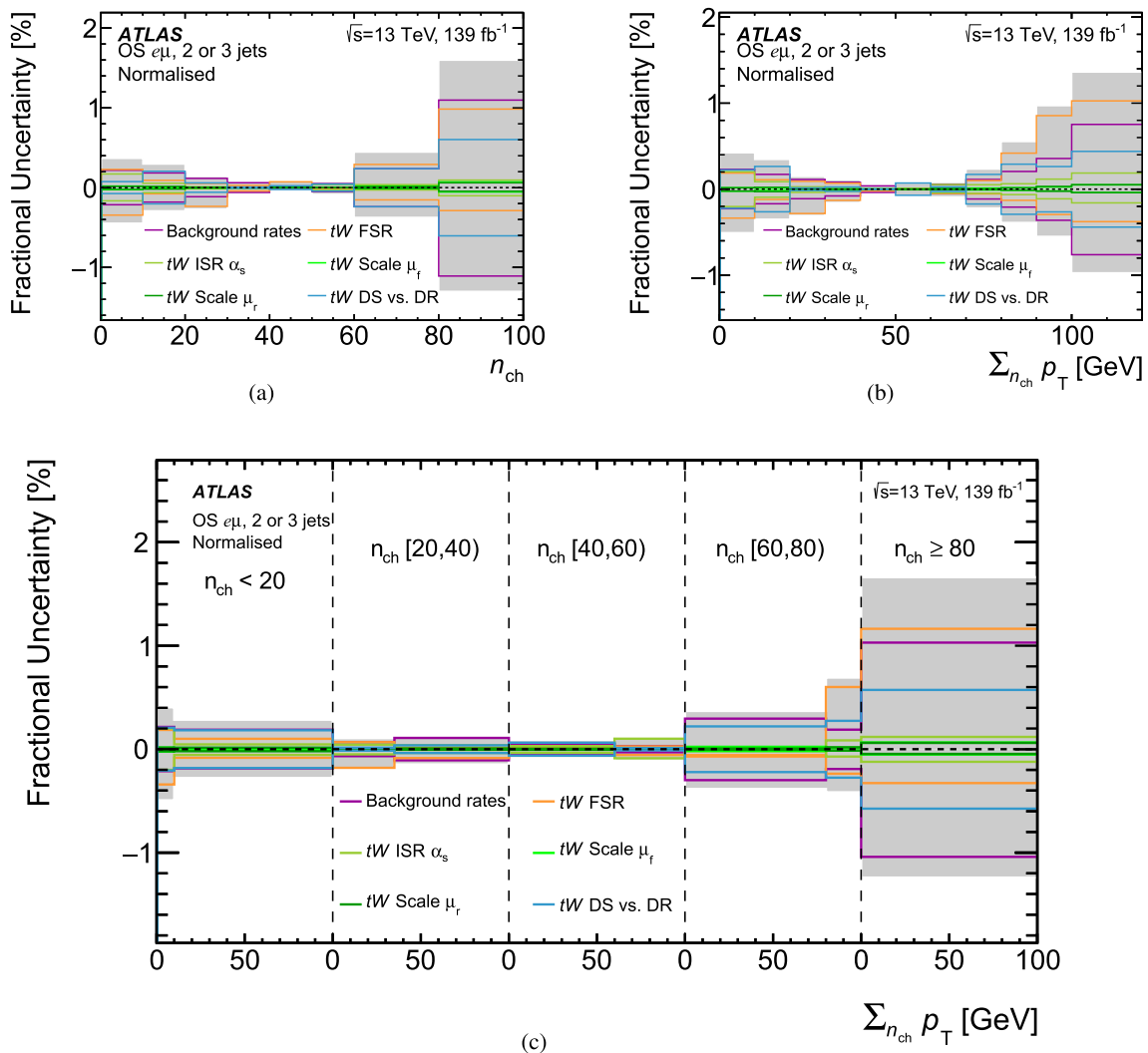
Fig. 6 Fractional uncertainties in the measured normalised differential cross-section as a function of a n_{ch} , b \sum_{n_{ch}} p_T , c \sum_{n_{ch}} p_T in bins of n_{ch} for event-based background rate uncertainties and modelling uncertainties for the tW process. The x -axis in c is split into five bins of n_{ch} by
