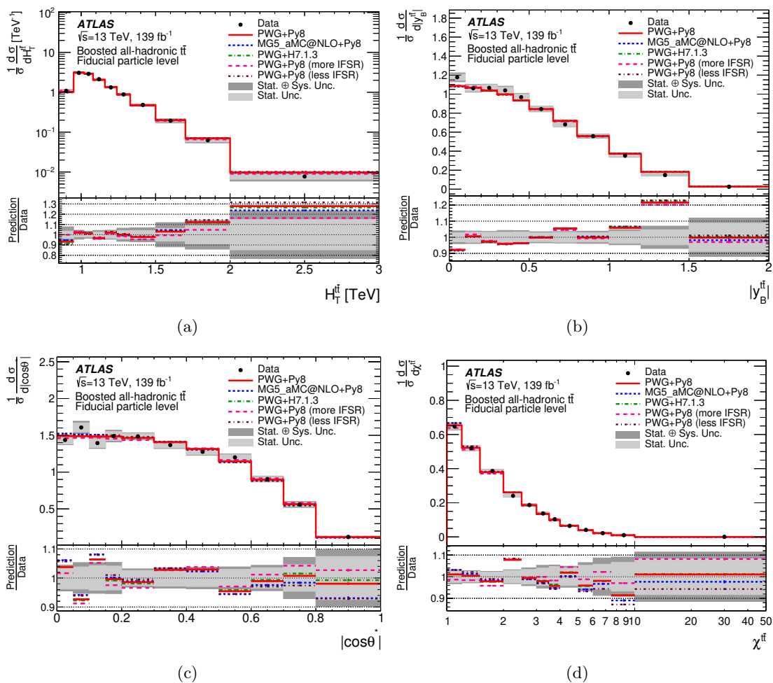
Figure 38. Normalized particle-level fiducial phase-space differential cross-sections as a function of (a) the scalar sum of the transverse momenta of the top-quark jets, (b) the t\bar{t} rapidity boost, (c) the production angle in the Collins–Soper reference frame, and (d) the production angle \chi^{t\bar{t}} . The dark and light grey bands indicate the total uncertainty and the statistical uncertainty, respectively, of the data in each bin. Data points are placed at the centre of each bin. The POWHEG+PYTHIA 8 MC sample is used as the nominal prediction to correct the data to particle level.
