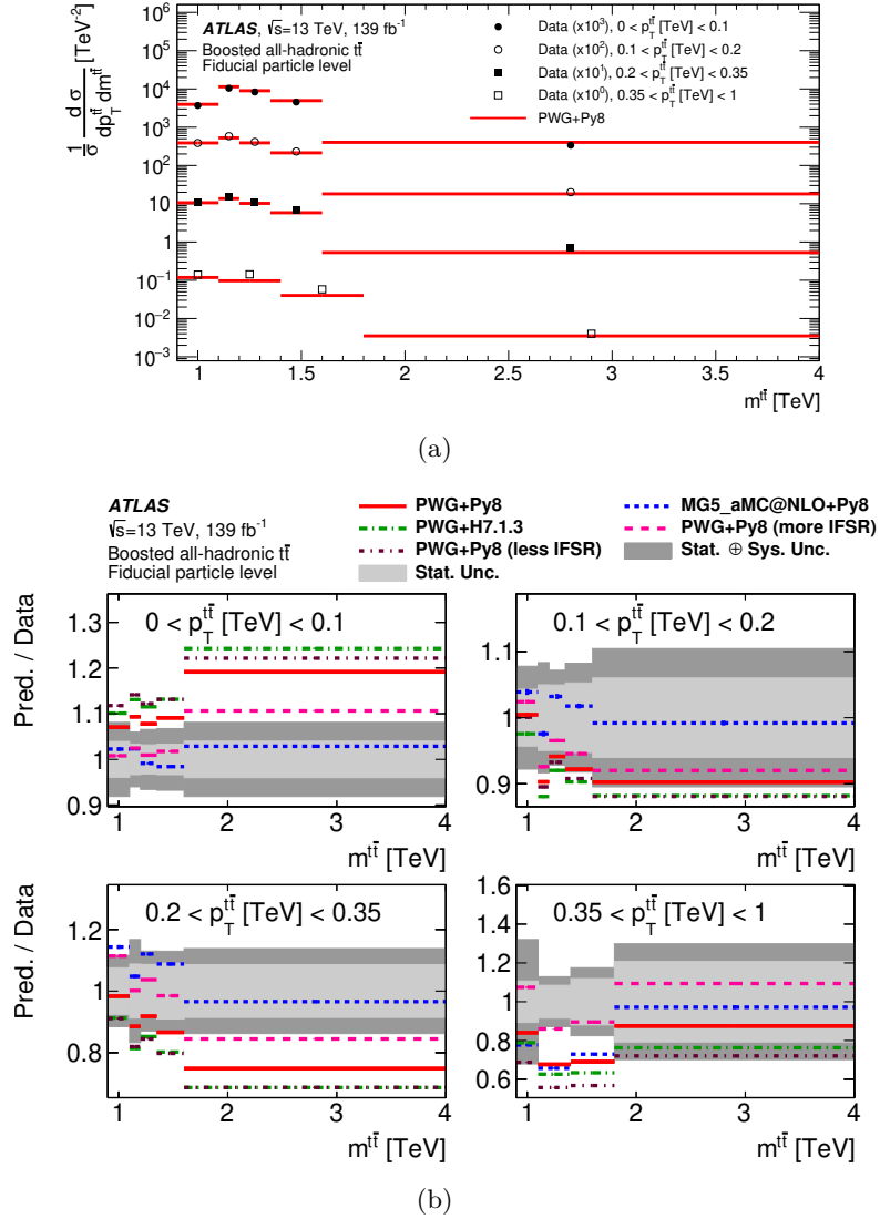
Figure 18. (a) Normalized particle-level fiducial phase-space double-differential cross-sections as a function of the p_T and the mass of the t\bar{t} final state, p_T^{tt} and m^{tt} , compared with the POWHEG+PYTHIA 8 calculation. Data points are placed at the centre of each bin and the POWHEG+PYTHIA 8 calculation is indicated by solid lines. The measurement and the prediction are normalized by the factors shown in parentheses to aid visibility. (b) The ratios of various MC calculations to the normalized particle-level fiducial phase-space differential cross-sections. The dark and light grey bands indicate the total uncertainty and the statistical uncertainty, respectively, of the data in each bin.
