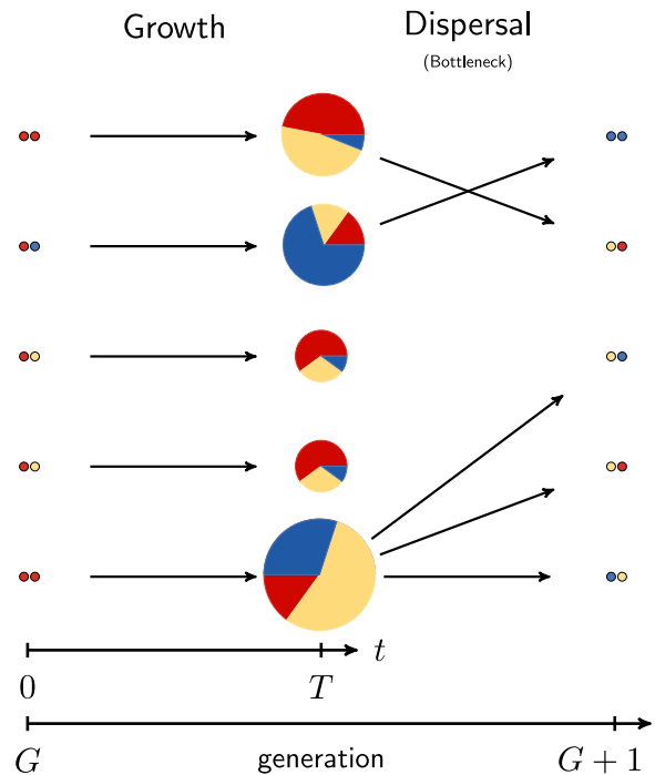
Fig. 1. Overview of the model and dynamics over a single generation for a population of M = 5 patches. Each patch is colonised by a small number of cells at t = 0 . A birth-death-mutation process then takes place (within-patch dynamics) over an interval of time [0, T] ; different colours represent the growth rates of different cell types that have distinct growth rates. The pie charts represent the total population of each of the M patches at dispersal. The size of slices in the pie charts represents the percentage of each type in the population and the overall size of the pies indicates the total relative population of the patch. After the growth phase, a dispersal event populates a fresh set of patches and, in doing so, creates a bottleneck, which (in this example) is a fixed size of two.
