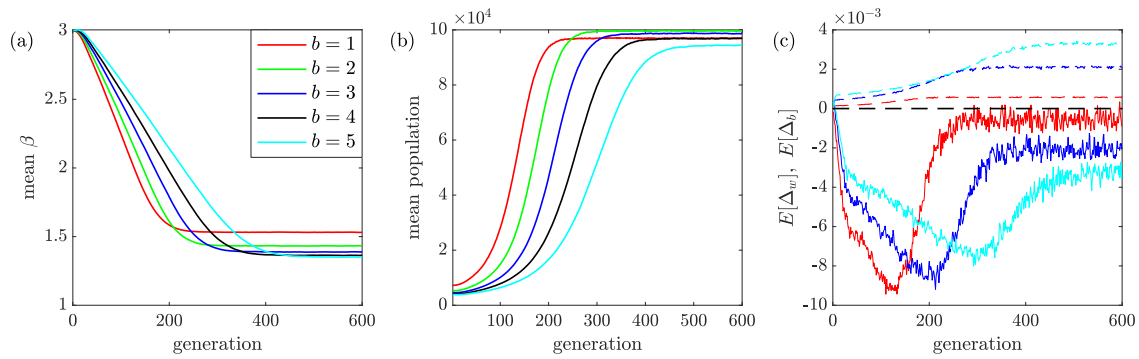
Fig. 5. Evolutionary dynamics for a system with varying bottleneck sizes. (a) The average growth rate, (b) the average total population per patch and (c) the average change in growth rate decomposed into within- (dashed lines) and between-patch (solid lines) components. Each line shows the averages over 50 individual realisations. Parameters: \mu = 0.05 , p = 0.01 , q = 0.5 , T = 10 , M = 100 .
