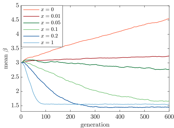
Fig. 10. Evolution in the mean growth rate, \beta , for a non-uniform, binary bottleneck distribution. Bottleneck sizes are drawn from a distribution where f_1 = x and f_{20} = 1-x with 0 \leq x \leq 1 . Thus, x = 1 corresponds to a strict unicellular bottleneck ( b = 1 ) and x = 0 a bottleneck of b = 20 .
