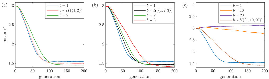
Fig. 9. The evolution of average growth rate when bottleneck size is chosen from a discrete distribution, where \mathcal{U}(A) is uniform over the set A . (a) and (b) show the dynamics for mixtures of smaller bottlenecks, (c) shows the effects of a distribution where the size is either large or unicellular.
