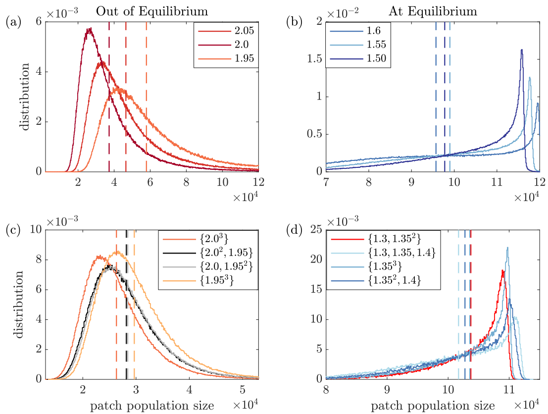
Fig. 6. Patch size distributions at the time of dispersal ( T = 10 ) for different initial growth rates and bottleneck sizes, both in an out of equilibrium. Panel (a) shows results for a single cell bottleneck out of equilibrium, and (b) at equilibrium ( \beta \approx 1.55 in this case). Panels (c) and (d) show the same quantities for a three-cell bottleneck. Note for b = 3 , the equilibrium growth rate is lower ( \beta \approx 1.35 ). In all panels, vertical dashed lines indicate the mean patch size for each distribution.
