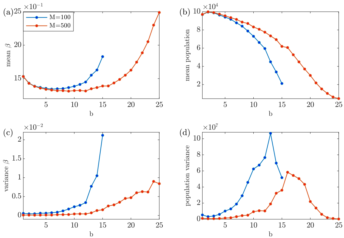
Fig. 8. The mean and variance of growth rate and patch size at equilibrium as a function of bottleneck size for M = 100 and M = 500 . (a) and (c) show the mean and variance in the cell growth rate. (b) and (d) show the same for the patch size. Note that the curve for M = 100 does not continue after b = 15 as there is no longer an equilibrium (see Fig. 7). Other parameters: \mu = 0.05 , q = 0.5 , p = 0.01 and T = 10 .
