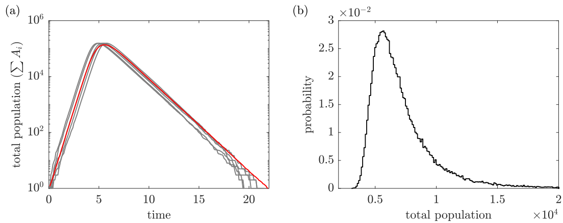
Fig. 2. Trajectories of cell populations within a patch. (a) The mean total population (red line) and five realisations of the total patch population as a function of time (grey lines). Patch population is computed as the sum of individual cells in a patch. Only five of the realisations are shown to more clearly illustrate the stochastic effects on the dynamics of the system. (b) The total size distribution estimated at t = 10 from 10^5 realisations. Other parameters: V = 10^6 , \bar{\beta} = \{3.0\} , p = 0.01 , q = 0.5 , \mu = 0.1 .
