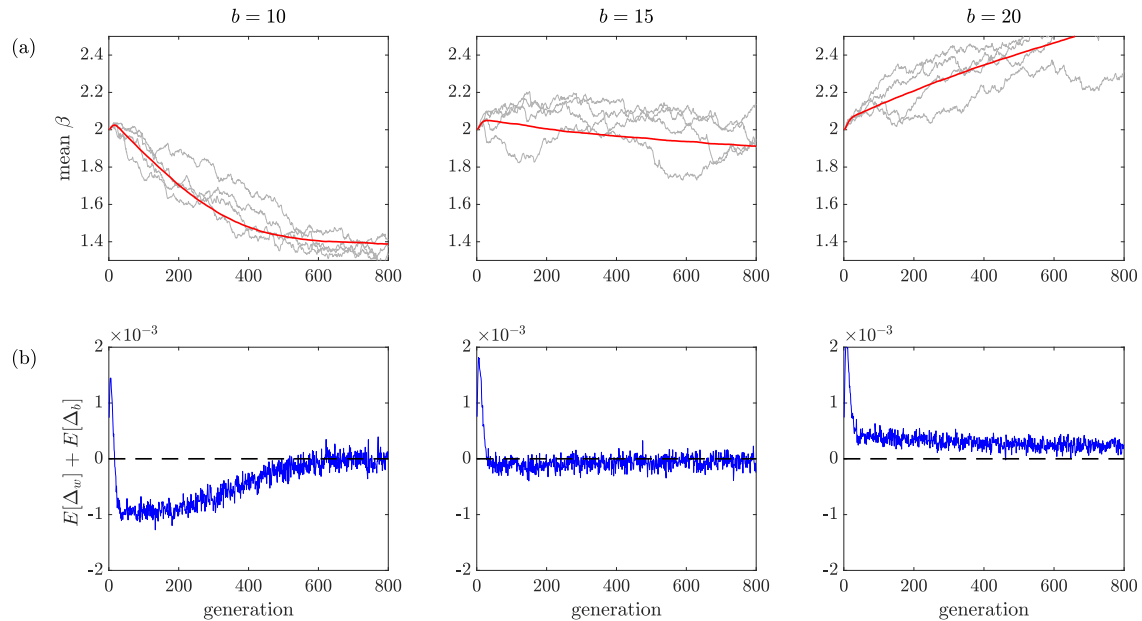
Fig. 7. Evolutionary dynamics with larger bottlenecks. (a) Change in the average growth rate over generations. (b) The sum of the within- ( \Delta_w ) and between-patch ( \Delta_b ) forces of selection, which illustrates the net force of selection (net change in the growth rate per generation, see Eq. (14)). For b = 10 and 15 , simulations eventually reach equilibrium; hence, the difference goes to zero. For b = 20 , within-patch selection always dominates between-patch selection and so the difference remains positive. Model parameters: M = 100 patches, \mu = 0.1 , p = 0.01 and q = 0.5 .
