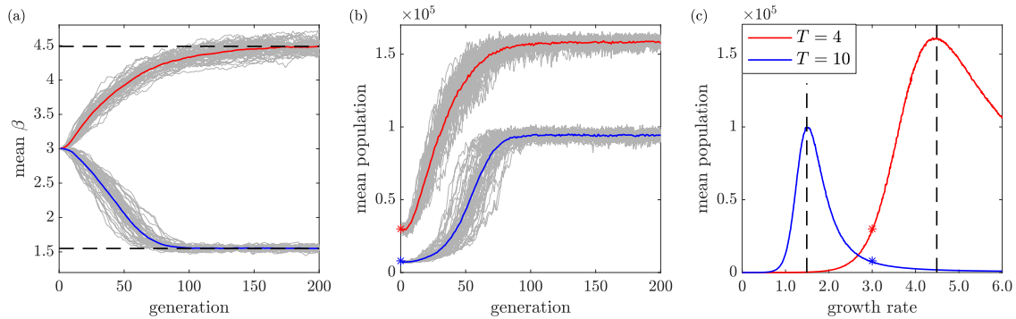
Fig. 4. Evolutionary dynamics for a system with a bottleneck of one cell, and for two different dispersal times, T = 4 and 10 . (a) The average growth rate over a population of 100 patches and (b) the average total population per patch. The grey lines show 50 individual realisations, and the coloured lines show the averages over these realisations. In both cases, the dispersal process creates a selection pressure that favours larger patches at the time of dispersal. Dashed lines show the equilibrium growth rates and the starred points represent patch population sizes for the initial growth rate of the simulations. (c) Fitness landscape view of the evolutionary process for fixed dispersal times T = 4 and 10 . Each curve shows the average total population within a patch for a fixed dispersal time as a function of the growth rate of the initial cell that colonises a patch. When T = 4 , the population peaks at a growth rate of \beta \approx 4.5 , and, when T = 10 , the maximum population is reached when \beta \approx 1.5 . These peaks, indicated by the dashed lines, correspond to the equilibrium growth rates reached by the simulations shown in (a). The starred points indicate the patch population sizes for the initial growth rate of the simulations as seen in (b).
