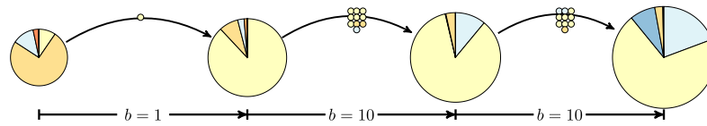
Fig. 11. Illustration of the homogenising effect of a randomly small bottleneck. If, by chance, a single slower growing cell is dispersed, this gains a larger advantage by freeing it from competition, which propagates through many subsequent generations.
