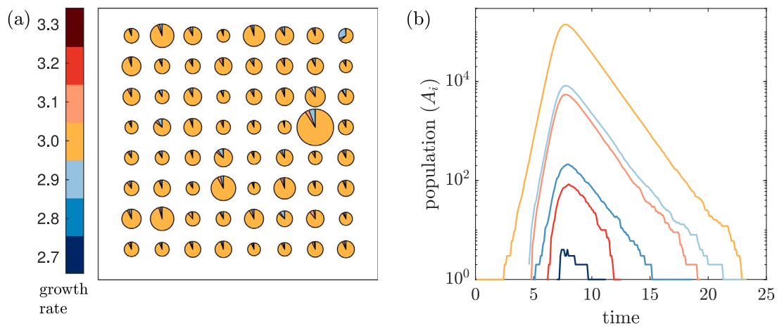
Fig. 3. Illustration of patch sizes and composition at dispersal. (a) 64 realisations of the within-patch model with the same initial conditions, \bar{\beta} = \{3.0\} , at dispersal time T = 10 . Each pie has area proportional to the total number of cells with arcs proportional to the composition. (b) A single realisation showing populations by type as a function of time over the growth phase. Both the pie charts and lines are coloured according to the growth rates for each cell type. Parameters are as in Fig. 2.
