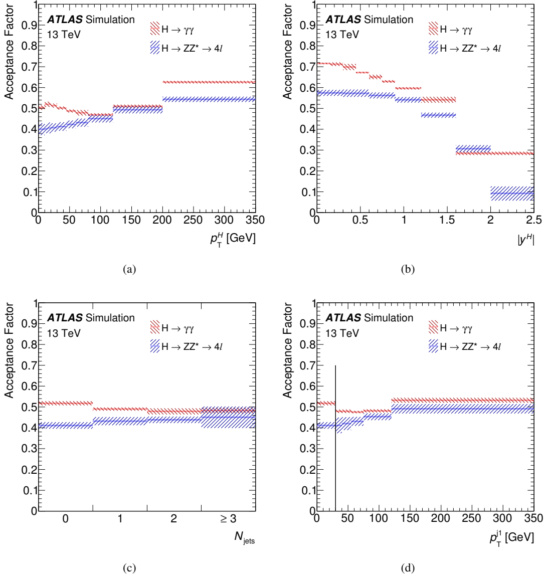
Figure 1: Acceptance factors for the extrapolation from the fiducial to the total phase space for the H \rightarrow \gamma\gamma decay channel (red) and the H \rightarrow ZZ^* \rightarrow 4\ell decay channel (blue), for (a) Higgs boson transverse momentum p_T^H , (b) Higgs boson rapidity |y^H| , (c) number of jets N_{\text{jets}} with p_T > 30 GeV, and (d) transverse momentum of the leading jet p_T^{j1} , including systematic uncertainties. The first bin in the p_T^{j1} distribution corresponds to the 0-jet bin in the N_{\text{jets}} distribution, as indicated by the black vertical line.
