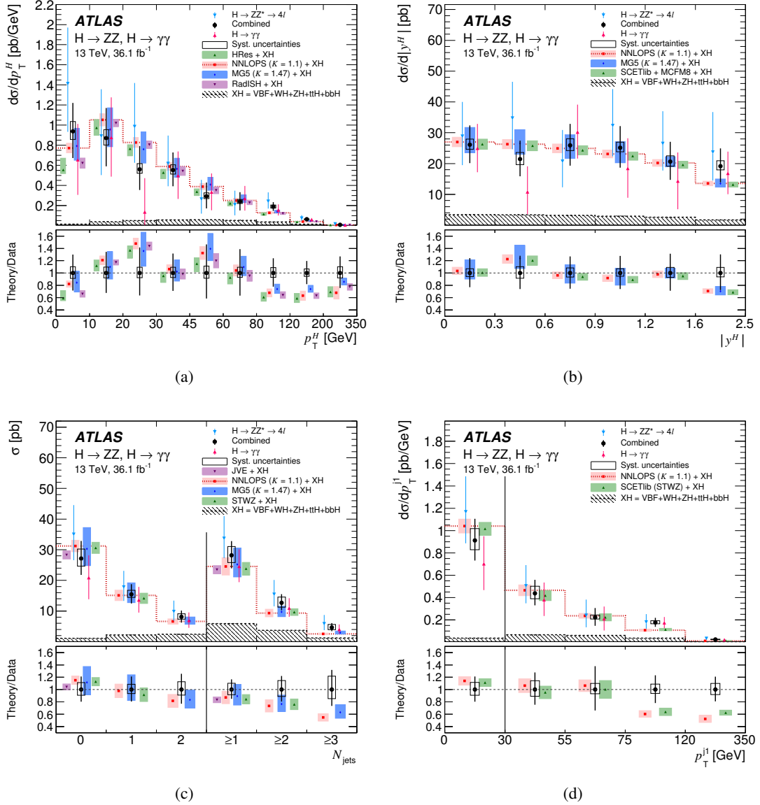
Figure 2: Differential cross sections in the full phase space measured with the H \rightarrow \gamma\gamma (red upward triangle) and H \rightarrow ZZ^* \rightarrow 4\ell (blue downward triangle) decay channels, as well as the combined measurement (black circle) for (a) Higgs boson transverse momentum p_T^H , (b) Higgs boson rapidity |y^H| , (c) number of jets N_{\text{jets}} with p_T > 30 GeV, and (d) the transverse momentum of the leading jet p_T^{j1} . The first bin in the p_T^{j1} distribution corresponds to the 0-jet bin in the N_{\text{jets}} distribution, as indicated by the black vertical line. Different SM predictions are overlaid, their bands indicating the PDF uncertainties as well as uncertainties due to missing higher-order corrections. The ordering of the predictions is the same in the legend as in the figure. Predictions for the other production processes XH are added to the ggF predictions, and also shown separately as a shaded area. The dotted red line corresponds to the central value of the NNLOPS ggF prediction, scaled to the total N 3 LO cross section by the given K -factor, and added to the XH prediction. The uncertainties due to higher orders in the NNLOPS prediction are obtained as in Refs. [11, 12, 78]. The MADGRAPH5_AMC@NLO prediction is scaled to the total N 3 LO cross section by the given K -factor. For better visibility, all bins are shown as having the same size, independent of their numerical width. The panel on the bottom shows the ratio of the predictions to the combined measurement. The total uncertainties of the combined measurement are indicated by the black error bars, the systematic uncertainties by the black open boxes.
