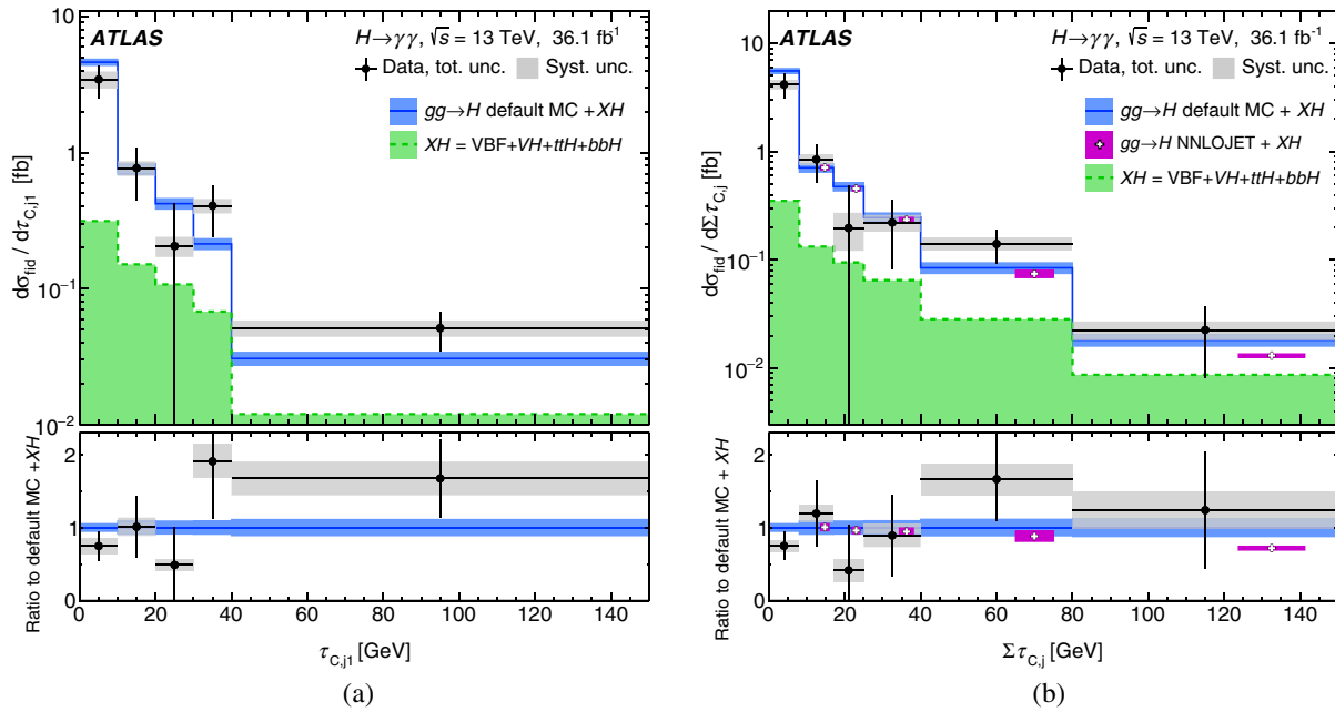
FIG. 38. The differential cross sections for pp \rightarrow H \rightarrow \gamma\gamma as a function of (a) \tau_{C,j1} and (b) \sum\tau_{C,j} are shown and compared to the SM expectations. The data and theoretical predictions are presented in the same way as in Fig. 36. In addition, the NNLOJET prediction is displayed in (b).
