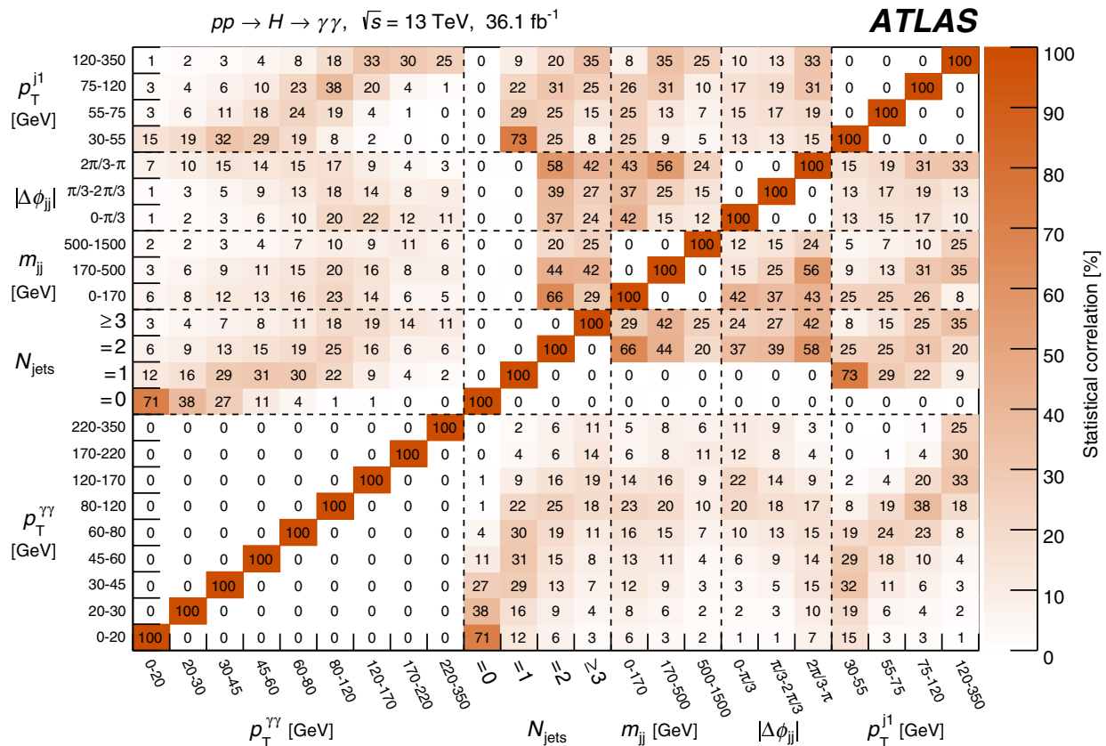
FIG. 20. The observed statistical correlations between p_T^{\gamma\gamma} , N_{\text{jets}} , m_{jj} , |\Delta\phi_{jj}| , and p_T^j are shown. These correlations were determined from an ensemble of 100,000 bootstrapped data sets which are each reanalyzed using an unbinned maximum-likelihood fit of the diphoton invariant mass spectrum to extract the correlations.
