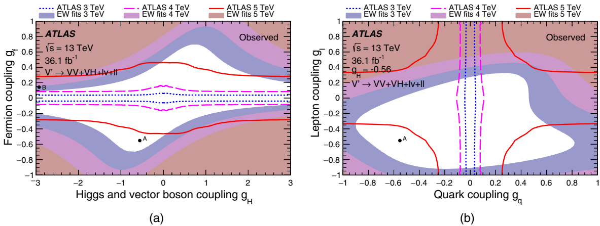
FIG. 11. Observed 95% C.L. exclusion contours in the HVT parameter space (a) \{g_H, g_f\} and (b) \{g_q, g_\ell\} for resonances of mass 3, 4, and 5 TeV for the combination of the VV , VH , and \ell\nu/\ell\ell channels. The areas outside the curves are excluded, as are the filled regions which show the constraints from precision EW measurements. Also shown are the parameters for models A and B, where applicable.
