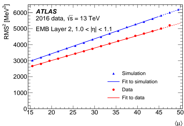
Figure 11. Evolution of the squared noise as a function of \langle \mu \rangle in data (red points) and simulation (blue triangles), for one particular \eta bin in the second layer of the EM calorimeter. The lines show the result of linear fits to the points for \langle \mu \rangle \in [15, 45] and the dotted lines show the extrapolation to higher \langle \mu \rangle .
