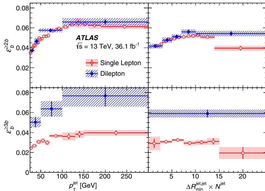
FIG. 4. Values of the per-jet b -tagging probability for t\bar{t} + \text{jets} events as a function of the jet transverse momentum ( p_T^{\text{jet}} ) and the minimum \Delta R between the considered jet and the other jets in the event, scaled by the jet multiplicity ( \Delta R_{\text{min}}^{\text{jet,jet}} \times N^{\text{jet}} ), as measured in data requiring the presence of at least two b -jets ( \epsilon_b^{\geq 2b} ) and least three b -jets ( \epsilon_b^{\geq 3b} ). b -tagging probabilities are shown separately for single-lepton and dilepton events. The vertical error bars indicate the statistical uncertainties, while the shaded (hatched) areas indicate the combined statistical and systematic uncertainties. In the dilepton case, a constant b -tagging probability is assumed as a function of \Delta R_{\text{min}}^{\text{jet,jet}} \times N^{\text{jet}} for \epsilon_b^{\geq 3b} .
