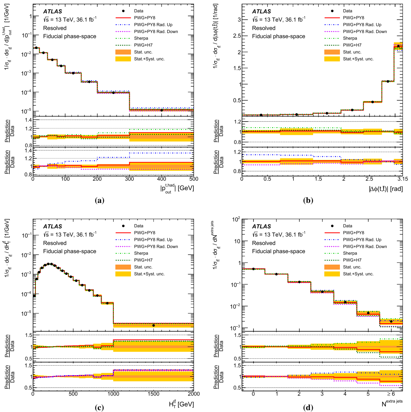
Fig. 25 Particle-level normalised differential cross-sections as a function of a |p_{out}^{t, had}| , b |\Delta\phi(t, \bar{t})| , c H_T^{tt} and d additional jet multiplicity in the resolved topology, compared with different Monte Carlo predic-
