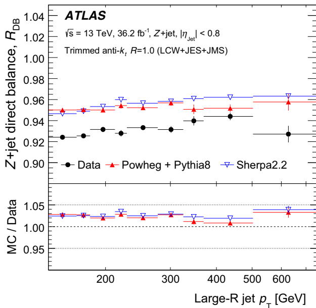
Fig. 7 The momentum balance R_{DB} as a function of the large- R jet transverse momentum p_T in Z+jet events for the combined e^+e^- and \mu^+\mu^- channels. Only statistical uncertainties are shown. For each p_T^{\text{ref}} bin, the measured R_{DB} is plotted against the average jet p_T of the bin. The horizontal error bars give an indication of the width of the associated p_T^{\text{ref}} bin
