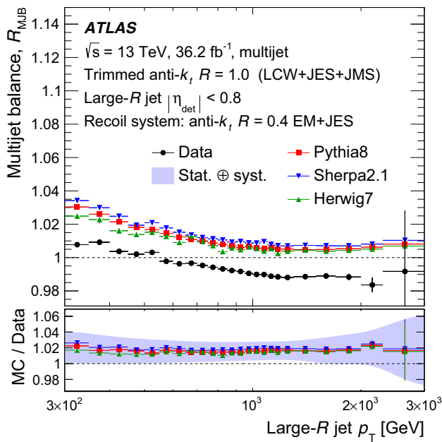
Fig. 12 Mean transverse momentum balance R_{\text{MJB}} for leading- p_T large- R jets ( |\eta| < 0.8 ) balanced against a system of at least two small- R jets ( p_T \geq 25 GeV, |\eta| < 2.8 ) as a function of the large- R jet transverse momentum p_T . The measured balance is compared with the prediction of Monte Carlo simulations based on the event generators PYTHIA 8, SHERPA 2.1, and HERWIG 7. Below, the ratio of response measurements in data and simulation is presented. The shaded band indicates the total uncertainty of the measurement, described in detail in the text. For each p_T^{\text{ref}} bin, the measured R_{\text{DB}} is plotted against the average jet p_T of the bin. The horizontal error bars gives an indication of the width of the associated p_T^{\text{ref}} bin
