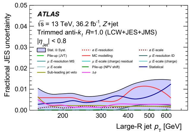
Fig. 8 Breakdown of the uncertainties in the JES measurement with the Z+jet direct balance method as a function of the large- R jet transverse momentum p_T . The sources include the statistical uncertainty, variations of the generator (simulation modelling), variations of the event selection (pile-up (JVT), sub-leading jet veto, \Delta\phi ), the uncertainties in the energy scale and resolution of electrons ( e E -scale and e E -resolution) and muons ( \mu E -scale and \mu E -resolution), and the uncertainty in the pile-up conditions ( N_{PV} shift). These uncertainties are also discussed in the context of small- R jets in Ref. [9]. The lines are obtained by smoothing a binned representation of these uncertainties using a sliding Gaussian kernel
