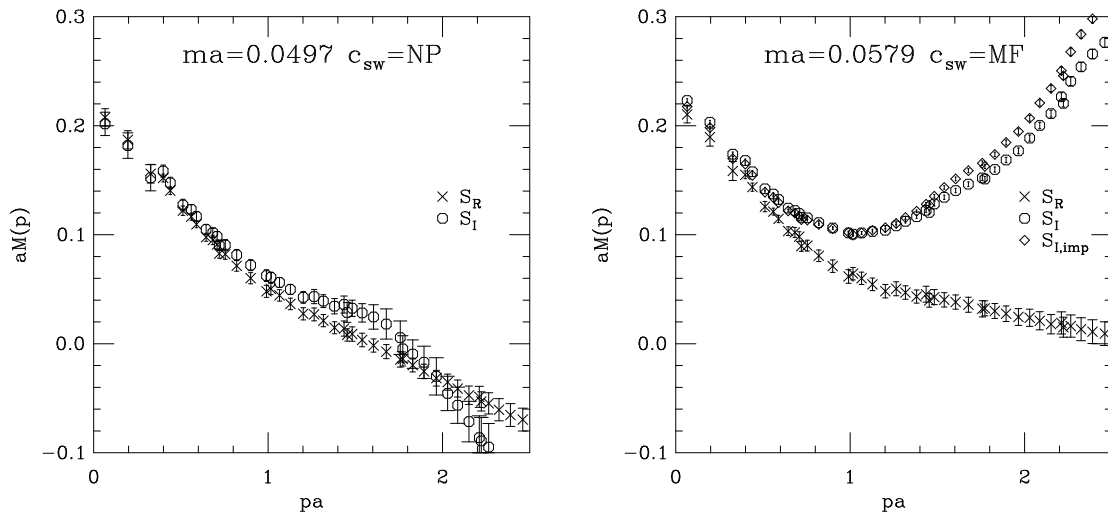
FIG. 2: The additively tree-level corrected mass function, for c_{sw} = NP , \kappa = 0.13344 (left) and c_{sw} = MF , \kappa = 0.13700 (right). S_{I,imp} in the right-hand figure is obtained using the mean-field improved rather than the tree-level values for b_q and \lambda in Eq. (2).
