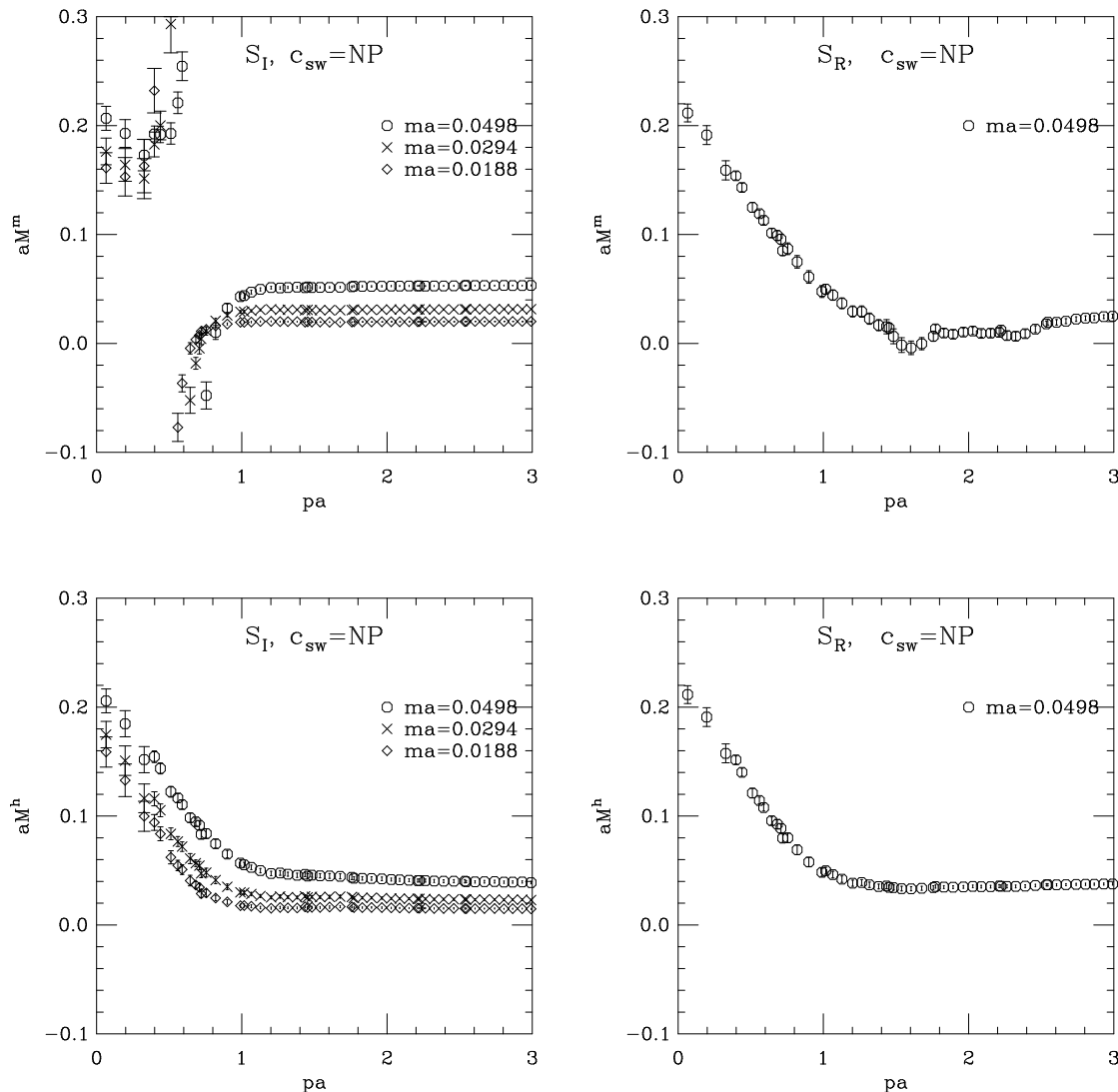
FIG. 5: The tree-level corrected M(p) , for c_{sw} = NP , using S_I (left) and S_R (right), and with the multiplicative (top) and hybrid (bottom) correction schemes. The multiplicative scheme clearly fails for S_I , and also performs poorly for S_R ; while the hybrid scheme performs well for both and leads to good agreement between the two propagators.
