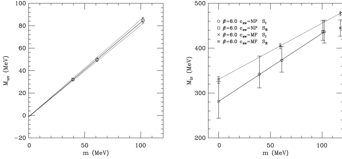
FIG. 7: Left: The ultraviolet quark mass M_{uv} as a function of the bare quark mass \tilde{m} , for S_I with c_{sw} = NP and using hybrid tree-level correction. The values are obtained by fitting M^h(p) to a constant for 2 < pa < 3 . Right: The infrared quark mass M_{ir} \equiv M(p=0) , obtained by extrapolating M(p) to pa = 0 , as a function of \tilde{m} . The bursts indicate the chirally extrapolated values of M_{ir} obtained by a simple straight line fit for each action. The solid line represents the fit for c_{sw} = NP , while the dotted line is the fit for c_{sw} = MF . We see that the values of M_{ir} from S_I and S_R agree for c_{sw} = NP , giving us further indication of the superiority of nonperturbative to mean-field improvement, despite the large statistical uncertainties in the NP data.
