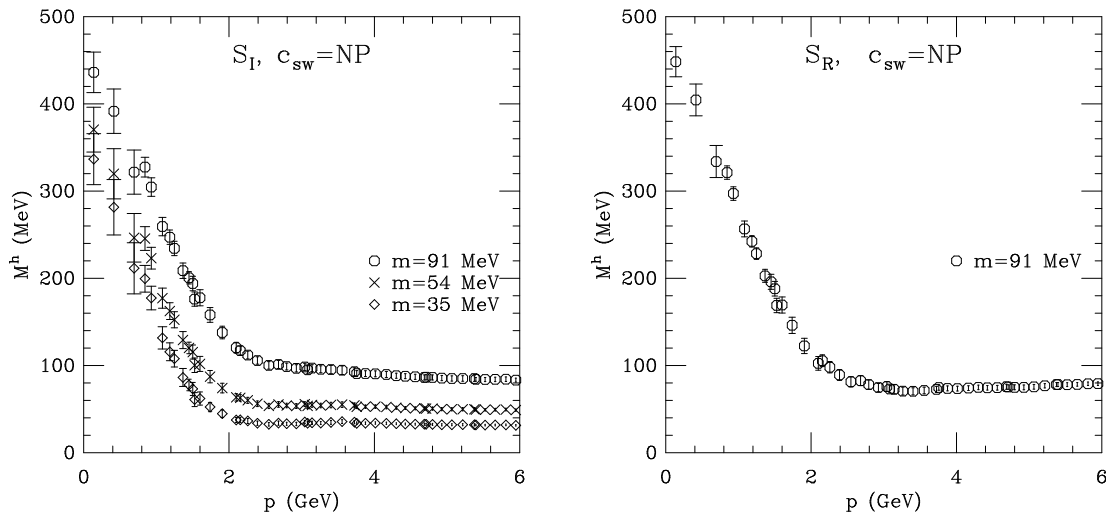
FIG. 6: The hybrid tree-level corrected M^h(p) , for c_{\text{sw}} = \text{NP} , using S_I (left) and S_R (right). For \tilde{m} = 91 MeV we find good agreement between the two data sets, both in the infrared and ultraviolet. The residual disagreement at intermediate momenta is a pointer to lattice artifacts that we have not brought under full control, even with nonperturbative improvement and hybrid tree-level correction.
