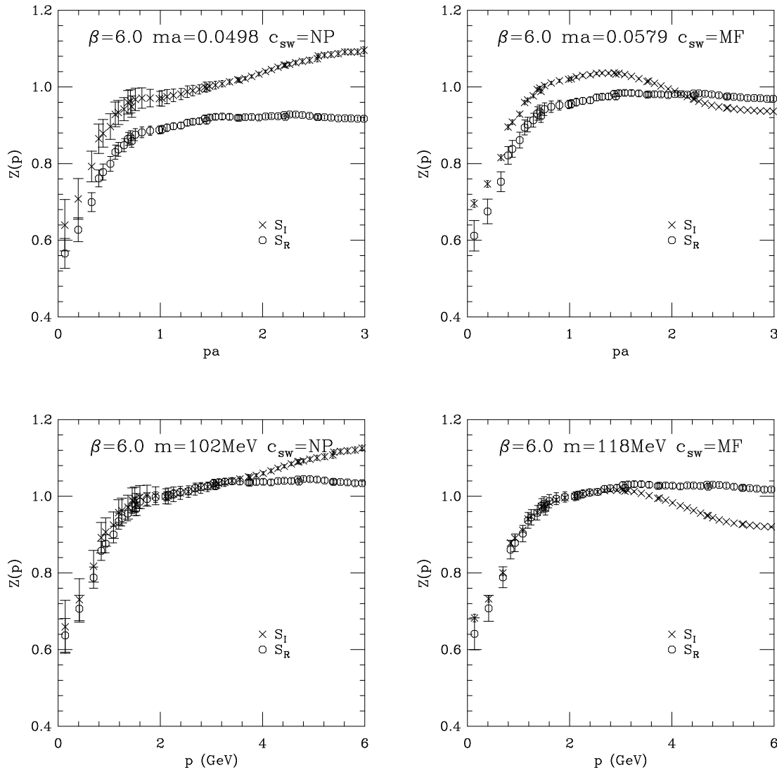
FIG. 4: The tree-level corrected Z(p) , for c_{sw} = \text{NP} , \kappa = 0.137 (left) and c_{sw} = \text{MF} , \kappa = 0.13344 (right). The upper two figures show the data in lattice units, and without rescaling. The lower two figures show Z(p) vs. momentum in physical units, and after rescaling (“renormalizing”) so that Z(2.1\text{GeV}) = 1 . The infrared agreement after rescaling is very good and we take the tree-level corrected Z(p) from S_R with the nonperturbative c_{sw} as the best estimate for this quantity (see text).
