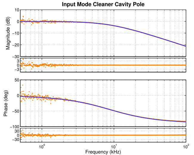
FIG. 11. The measured IMC cavity pole is shown together with a simple single pole fit and the fit residuals.
