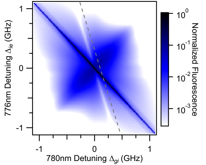
FIG. 8. Model 3: Excited-state population, P_e , for the population pumping model. Model parameters were \Omega_{gi,\pm} = \Gamma_i and \Omega_{ie,+} = \Gamma_i/10 . LD_{-1} , L_{\pm 1} , and L_{-3} lines are all generated. The dashed line has a gradient of -3 .
