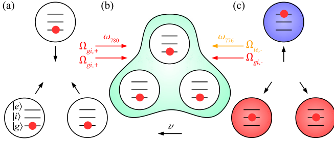
FIG. 3. Hypothesis 1: A proposed resonant process involving the collision of three atoms. Three atoms in their ground states collide (a) to form a metastable triatomic molecule (b). The molecule absorbs four photons, three from the \omega_{780} field and one from the \omega_{776} field, and decays into two singly excited atoms and one double-excited atom (c).
