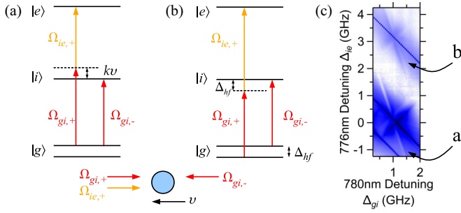
FIG. 7. Hypothesis 3: Optical pumping for (a) the strong stepwise transition and (b) the shadow observed in the other ground state both highlighted in the data (c). Detunings from the intermediate state are shown (not to scale) where kv is a detuning of a Doppler shift and \Delta_{hf} is ground-state splitting of Rb being \approx 3 and \approx 6 GHz for the ^{85}\text{Rb} and ^{87}\text{Rb} isotopes, respectively.
