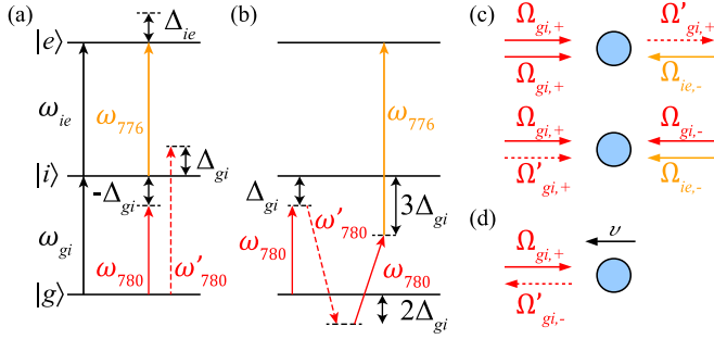
FIG. 5. Hypothesis 2: A proposed resonant, Doppler-free, four-photon process. (a) Atoms are illuminated with light at frequencies \omega_{780} and \omega_{776} . We further hypothesize the existence of another field at \omega'_{780} , but with the opposite detuning to the imposed field \omega_{780} ; a mechanism for the autonomous, resonant production of this field is described in the text. (b) Resonant four-photon transition in which two \omega_{780} photons and one \omega_{776} photon are absorbed, accompanied by stimulated emission of a photon into the \omega'_{780} field. (c) Configurations of four beams that produce Doppler-free transitions. (d) Seeding the ancillary field \omega'_{780} by backscattering the applied field \omega_{780} from a Doppler-resonant atom; the stimulated process in panel (b) will then self-consistently amplify the seed field.
