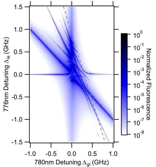
FIG. 4. Model 1: Excited state populations, P_e , for the triatomic collision model. Here we take \Omega_{ie,-} = \Omega_{gi,+}/100 , \Omega_{gi} \gg \Gamma_{ab} , and v_{ie}/r_{jk}^3 = 8 as arbitrary but illustrative quantities. We have shown only the stationary, v = 0 , velocity class. The dashed line has a gradient of -3 .
