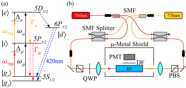
FIG. 1. (a) Energy level diagram of the two-photon transition. Solid arrows are driving lasers; dashed arrows show decay routes. (b) Schematic of the optical experimental setup. SMF, single mode fiber; PBS, polarizing beam splitter; QWP, quarter wave plate; DF, dichroic filter.
