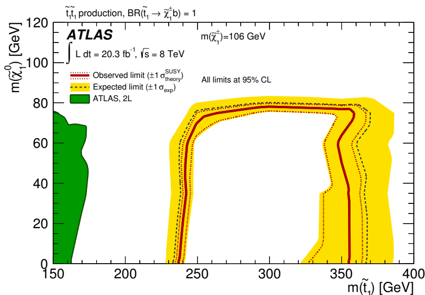
Figure 20. Observed and expected exclusion contours at 95% CL in the (\tilde{t}_1, \tilde{\chi}_1^0) mass plane for a fixed value of m(\tilde{\chi}_1^+) = 106 \text{ GeV} . The dashed and solid lines show the 95% CL expected and observed limits, respectively, including all uncertainties except for the theoretical signal cross-section uncertainty (PDF and scale). The band around the expected limit shows the \pm 1\sigma expectation. The dotted \pm 1\sigma lines around the observed limit represent the results obtained when moving the nominal signal cross-section up or down by the theoretical uncertainty. The solid green area shows the excluded region from a previous ATLAS two-lepton analysis [20].
