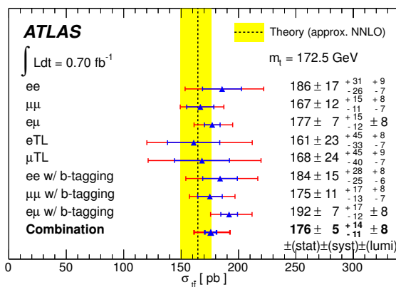
Figure 3. Summary of the individual cross section measurements and the combination of non- b -tag and exclusive b -tagged results. The vertical dashed line and yellow band are the approximate NNLO theory calculation and its uncertainty.
