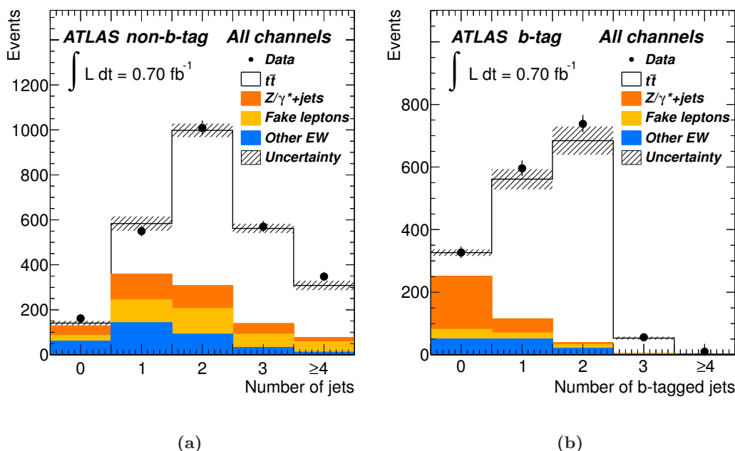
Figure 1. (a) Jet multiplicity distribution for ee+\mu\mu+e\mu+e\text{TL}+\mu\text{TL} events without a b -tagging requirement. (b) Multiplicity distribution of b -tagged jets in the ee+\mu\mu+e\mu channels. Contributions from diboson and single top-quark events are summarized as ‘Other EW’. The events in (b) are not a simple subset of those in (a) because the event selections for the b -tag and non- b -tag analyses differ. Uncertainties shown are statistical and systematic combined. The distributions are shown as stacked histograms.
