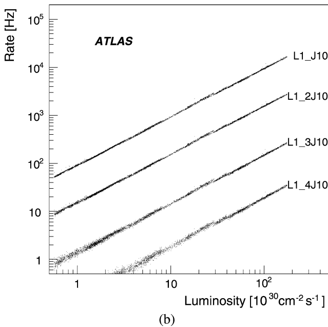
Fig. 44 Rates for various L1 jet triggers as a function of the instantaneous luminosity during the 2010 run for (a) inclusive triggers and (b) multi-jet triggers (with the inclusive trigger L1_J10 for reference)
